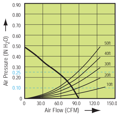
RAD80LED Fan Curve
