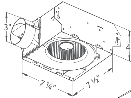
Fan Housing
